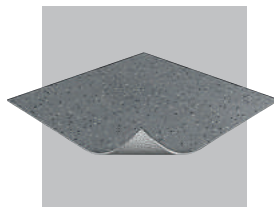
TOUCHDOWN PVC floor protection total weight: 2.2kg/m2 total thickness: 1.45mm 2m x 22 lm
